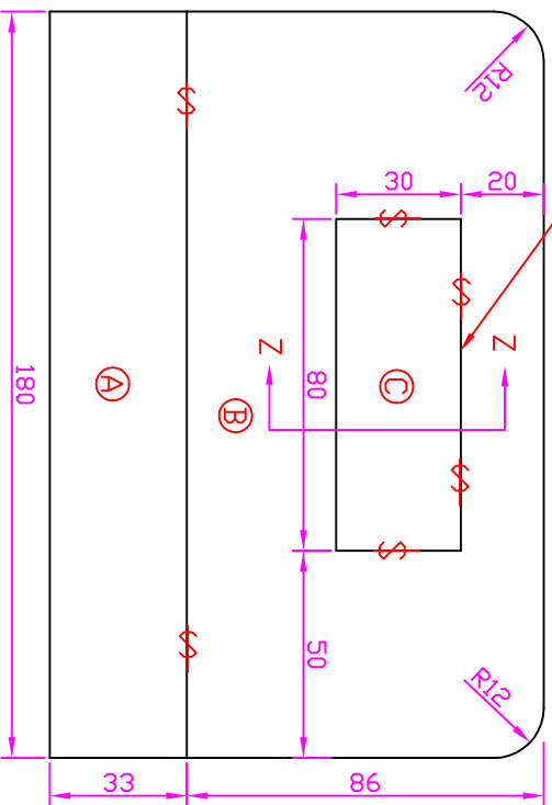
View -B (Side Panel)
